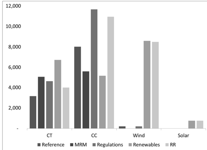
Figure 4. New Generation Capacity by Type 2015-2024 (MW)
