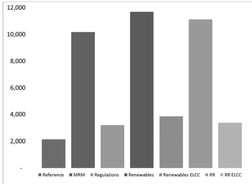
Figure 6. Net Capacity Additions 2015-2024 (MW)
