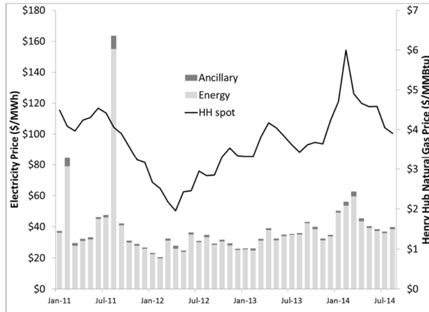
Figure 1. Average Price of Electricity in ERCOT
