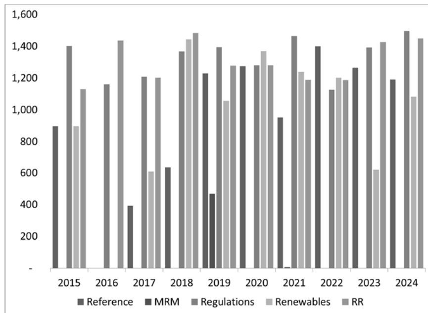
Figure 3. Retirements 2015-24 (MW)
