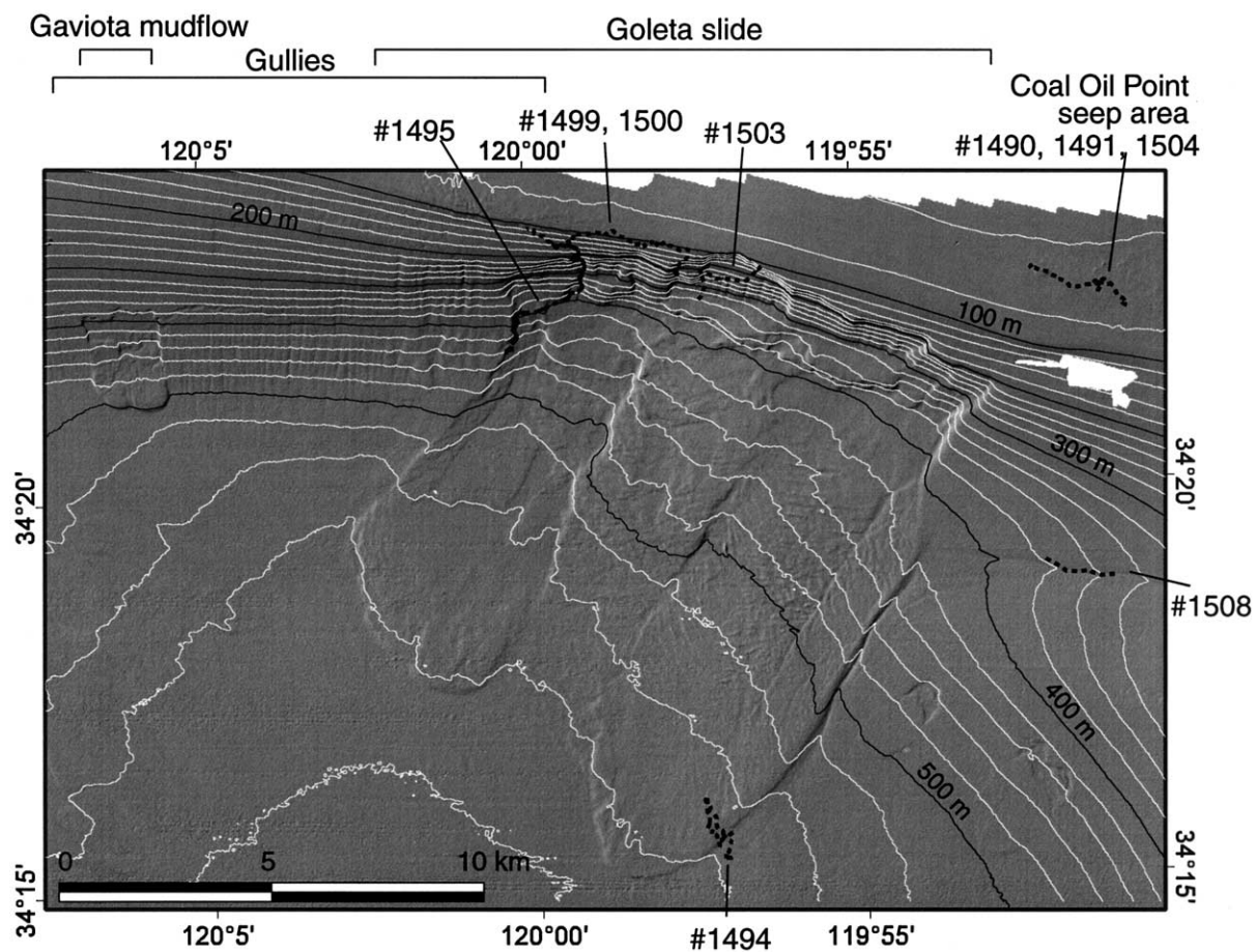
Fig. 7. Shaded relief image of mass wasting on the northern basin slope. Four-digit numbers and dotted lines indicate MBARI ROV Ventana dives.
