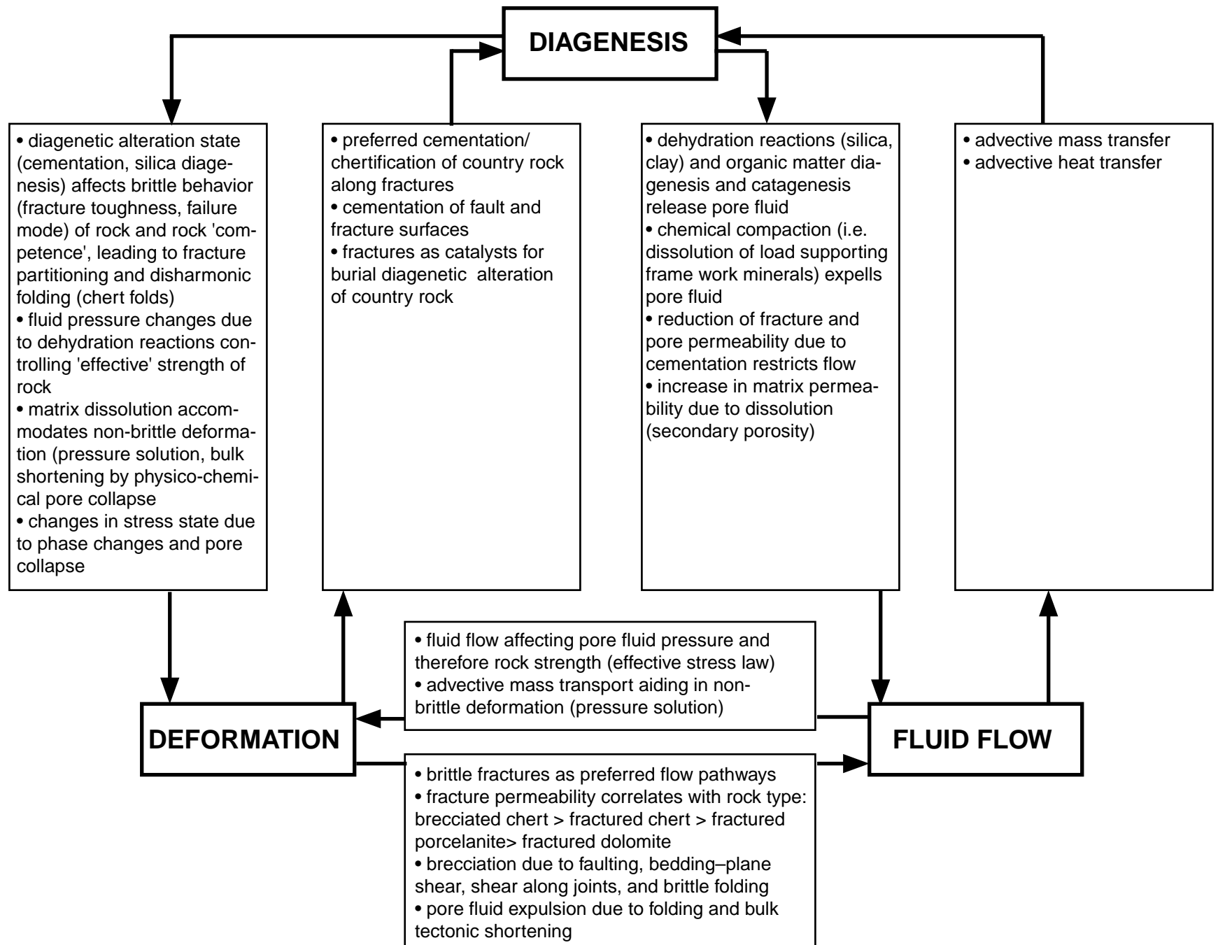
Figure 1: Potential relations among diagenesis, deformation, and fluid flow as applicable to the Monterey Formation.
