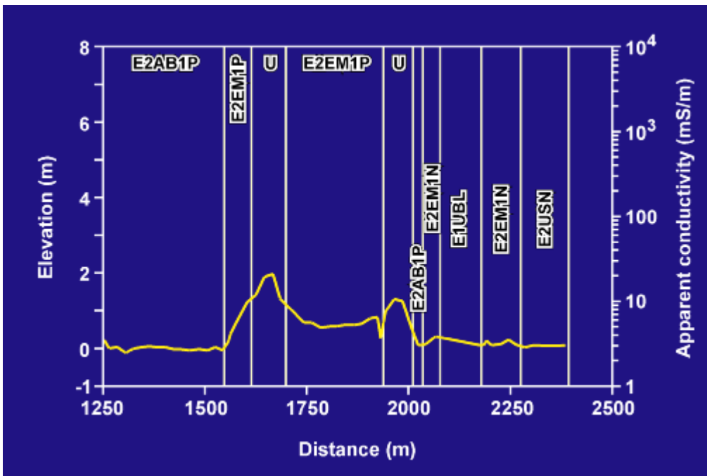
Figure 11. Relationship between soil conductivity, elevation, and habitat type along a transect on Mustang Island near Port Aransas. Habitats are from USFWS NWI maps based on 1992 aerial photos. From Paine et al. 2004.
