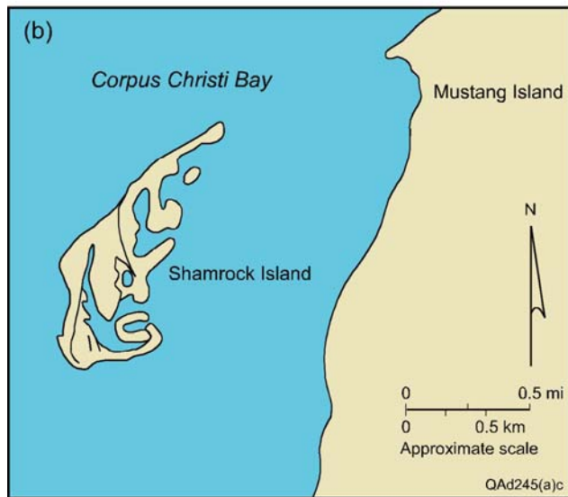
Figure 39. Illustration depicting how Shamrock Island grew as a compound recurved spit on the bayward side of Mustang Island, as shown in (a) on the basis of a 1958 aerial photo, and eventually was cut off from Mustang Island by Hurricane Celia in 1970; today it is an island (b). Also see Figures 40 and 41.
