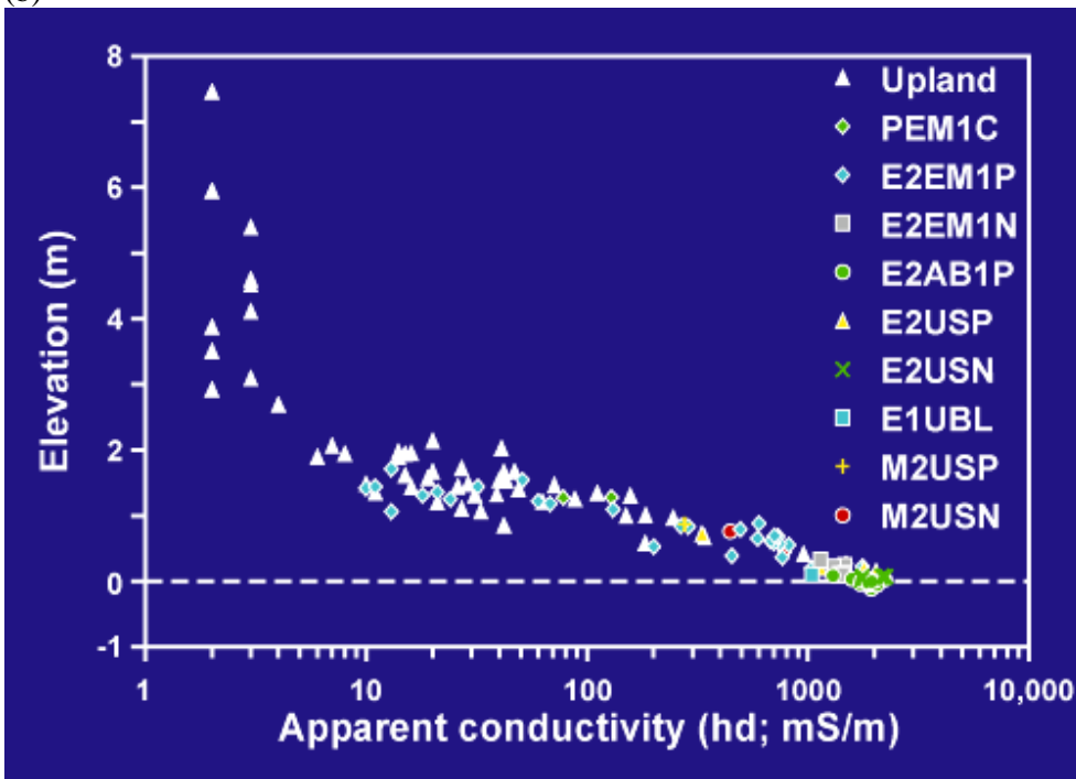
Figure 10. Digital elevation model (DEM) of a transect near Port Aransas showing habitats identified on USFWS NWI (1992) maps (a), and relationship between elevation, conductivity, and habitats along transects (b). The DEM was constructed from Lidar data acquired along the transect in 2003. From Paine et al. 2004a and b, 2005.
