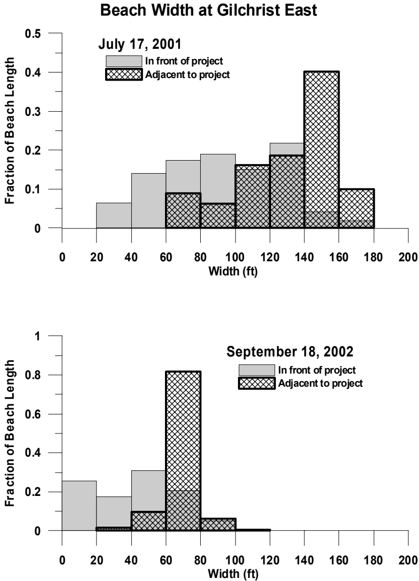
Figure 14. July 2001 and September 2002 beach width comparisons shown as fractions of beach length in front of and adjacent to the Gilchrist East (Gilchrist) geotextile tubes.
