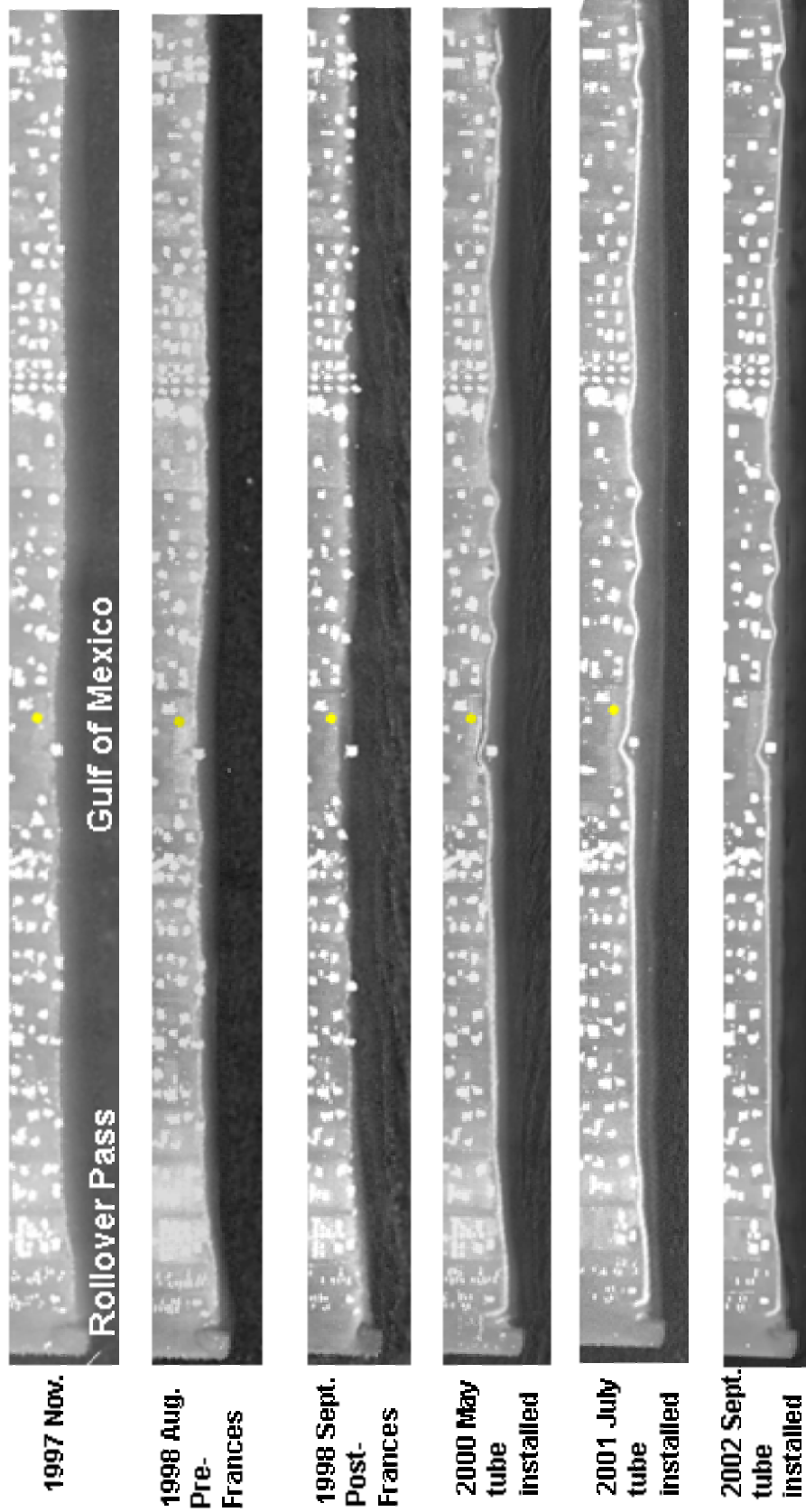
Figure 29. Lidar topographic images of a portion of the Gilchrist East project. Dark areas are low elevation, lighter higher elevation. Geotextile tubes were present during the 2000, 2001, and 2002 surveys. Note how the tubes were routed seaward of some houses and the overall geomorphic impact of the project.
