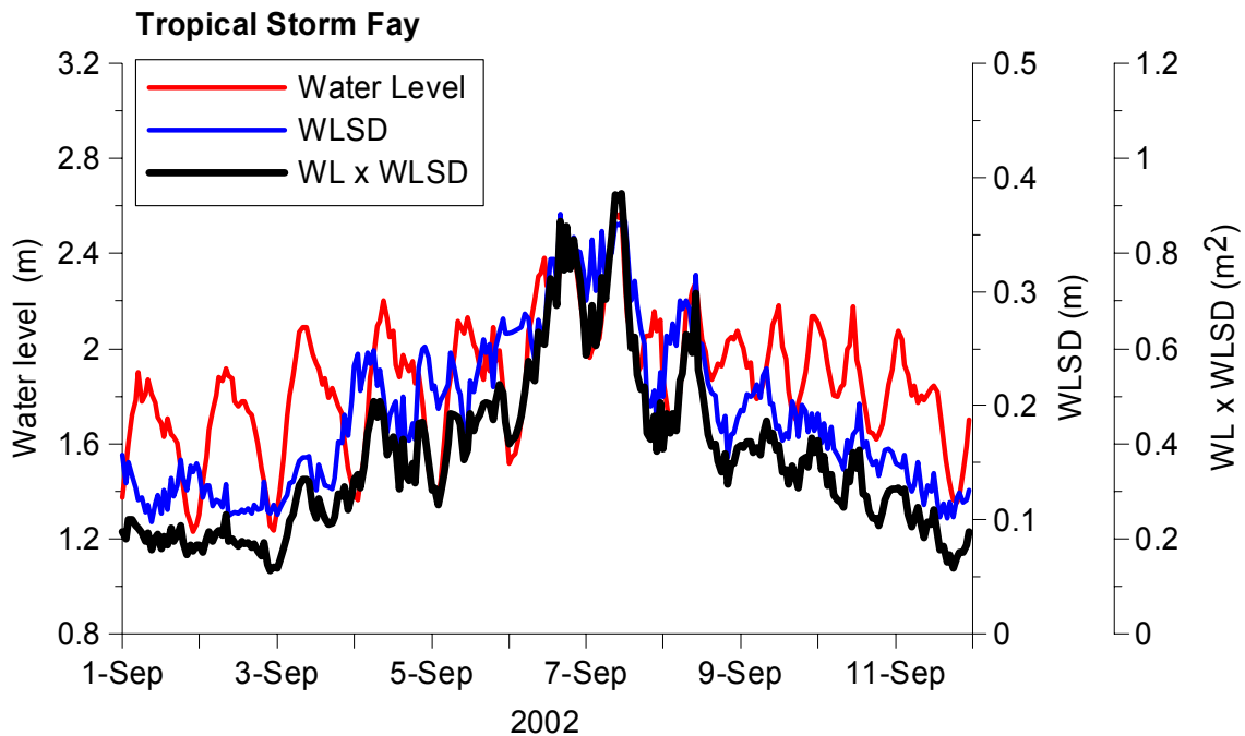
Figure 12. Water level (WL) and wave conditions represented by the water level standard deviation (WLSD) during Tropical Storm Fay. Data recorded by the Pleasure Pier tide gauge. WL is relative to the tide station's datum.
